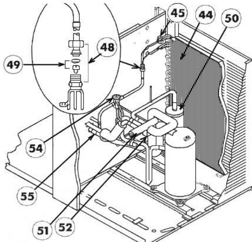
Condenser Assembly 036 On or After 5295
