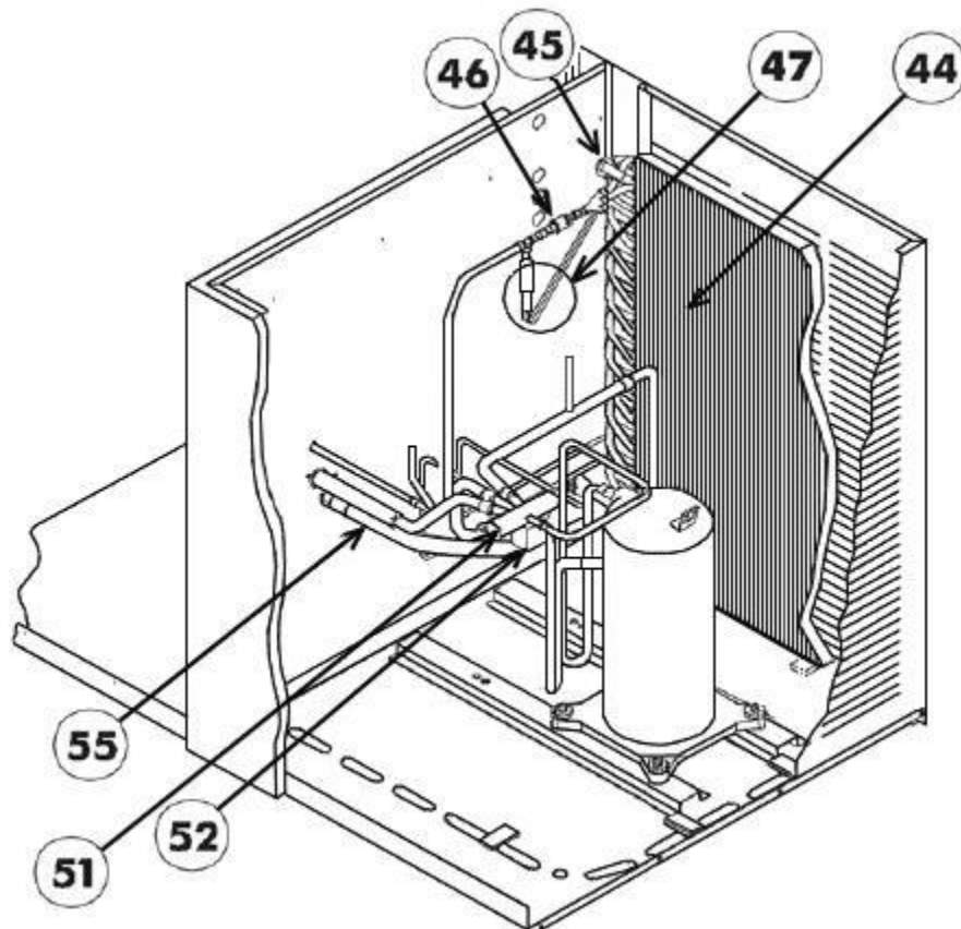
Condenser Assembly 018-024 On or Before 5195
