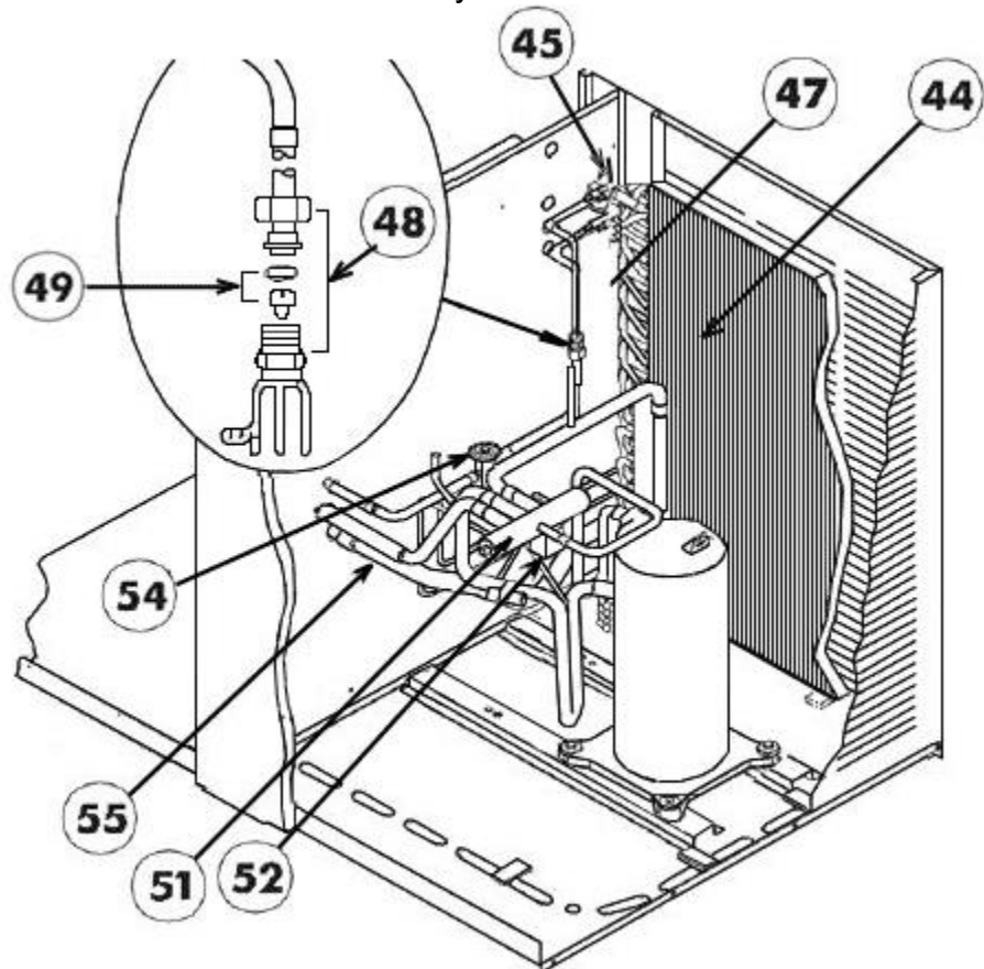
Condenser Assembly 018-030 On or After 5295
