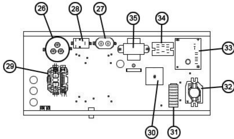
Control Box
