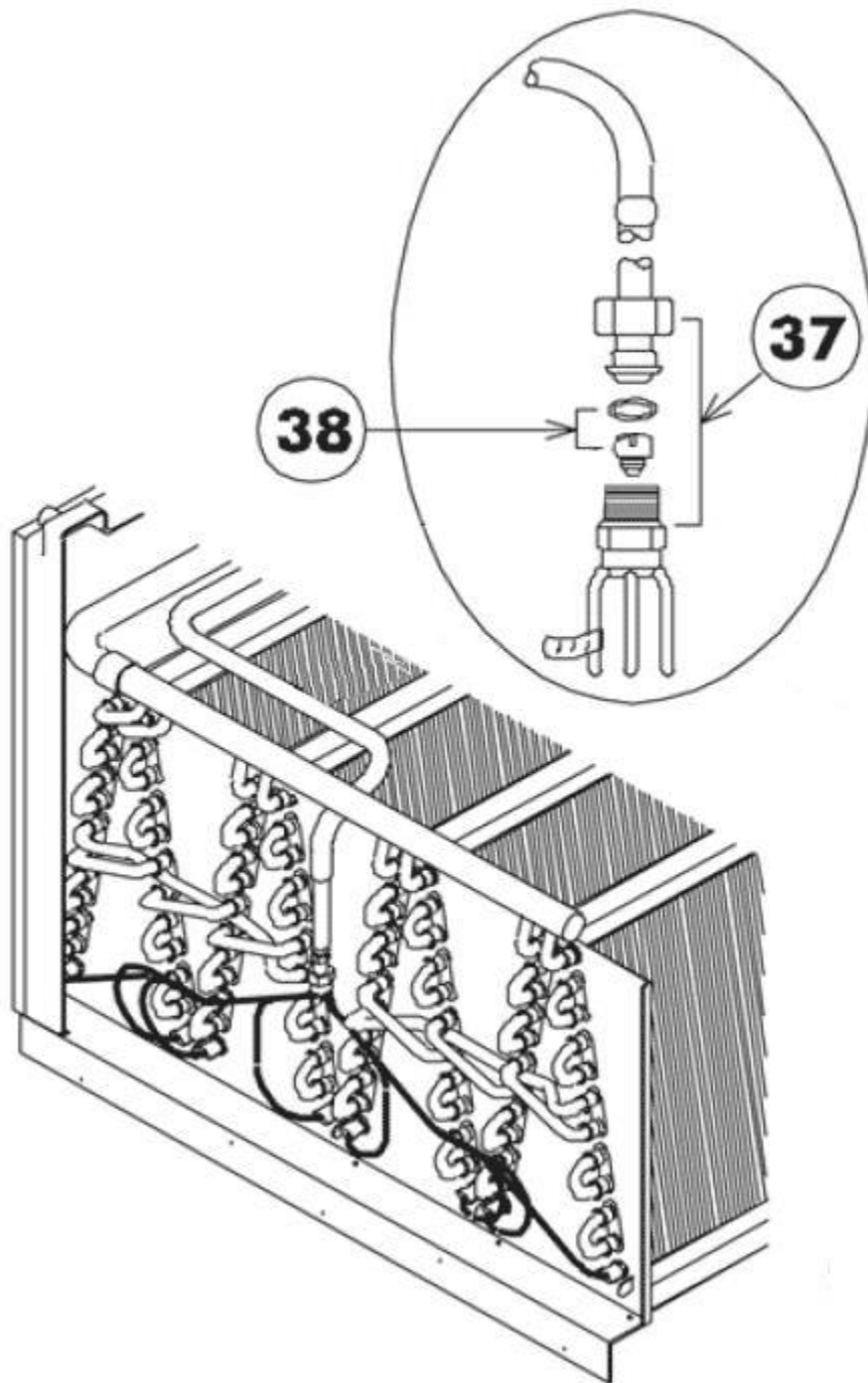
Evaporator Coil Assembly Cap Tube Metering Device
