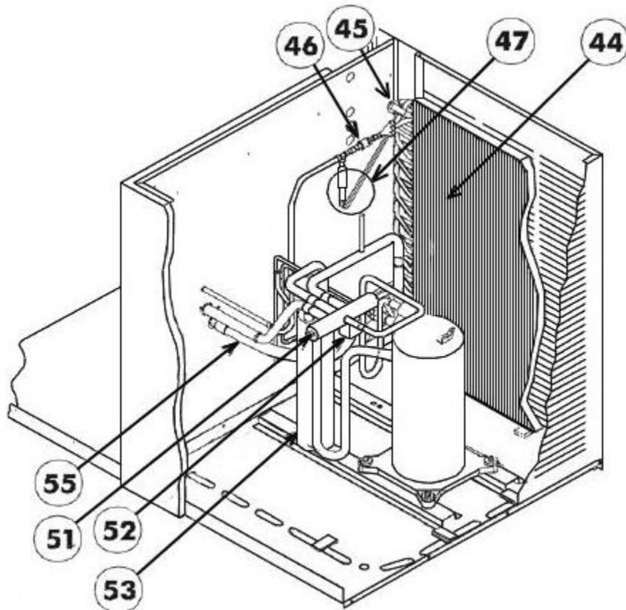
Condenser Assembly 030 On or Before 5195
