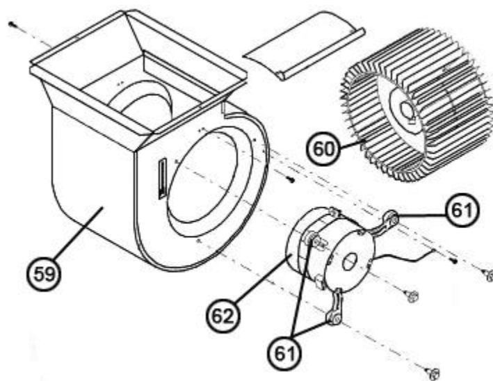
Blower Assembly
