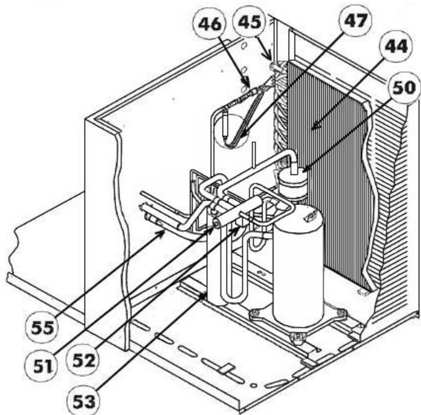
Condenser Assembly 036 On or Before 5195
